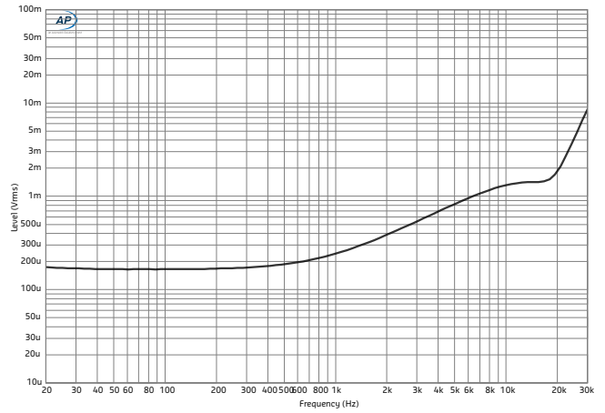
Output impedance, measured at output terminals
